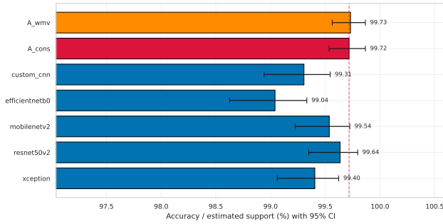
Figure 4: Full test-split accuracy (Wilson 95% CI) against the human-support estimands A_{\text{cons}} and A_{\text{wmv}} (stratified bootstrap 95% CI; dashed line = A_{\text{cons}} ).
