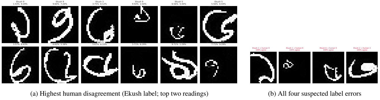
Figure 3: (a) The twelve items with the highest human label entropy. (b) The four suspected mislabels: stored label, human reading and panel agreement. The two right-hand items in (b) are the confident-learning candidates; the two 1→9 errors were missed by confident learning.
